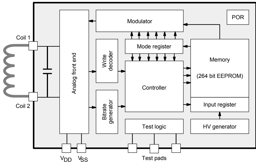
Figure 3. Block Diagram
