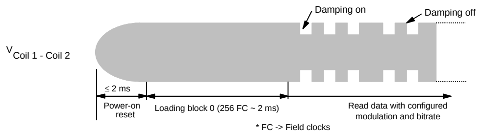
Figure 8. Voltage at Coil1/Coil2 After Power-on
