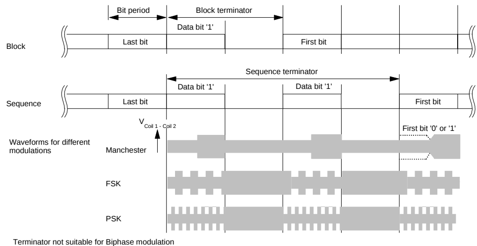
Figure 9. Terminators
