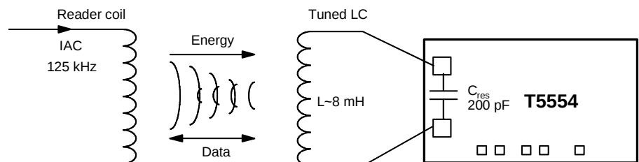
Figure 7. Application Circuit
