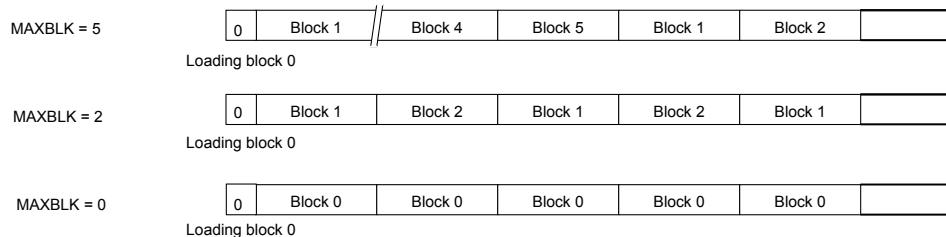
Figure 11. MAXBLK Examples
