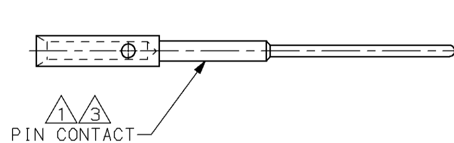
PIN CONTACT
