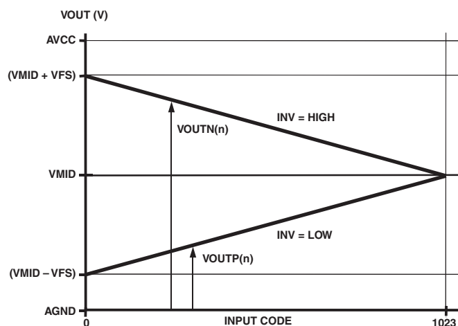
Figure 5. Transfer Function
