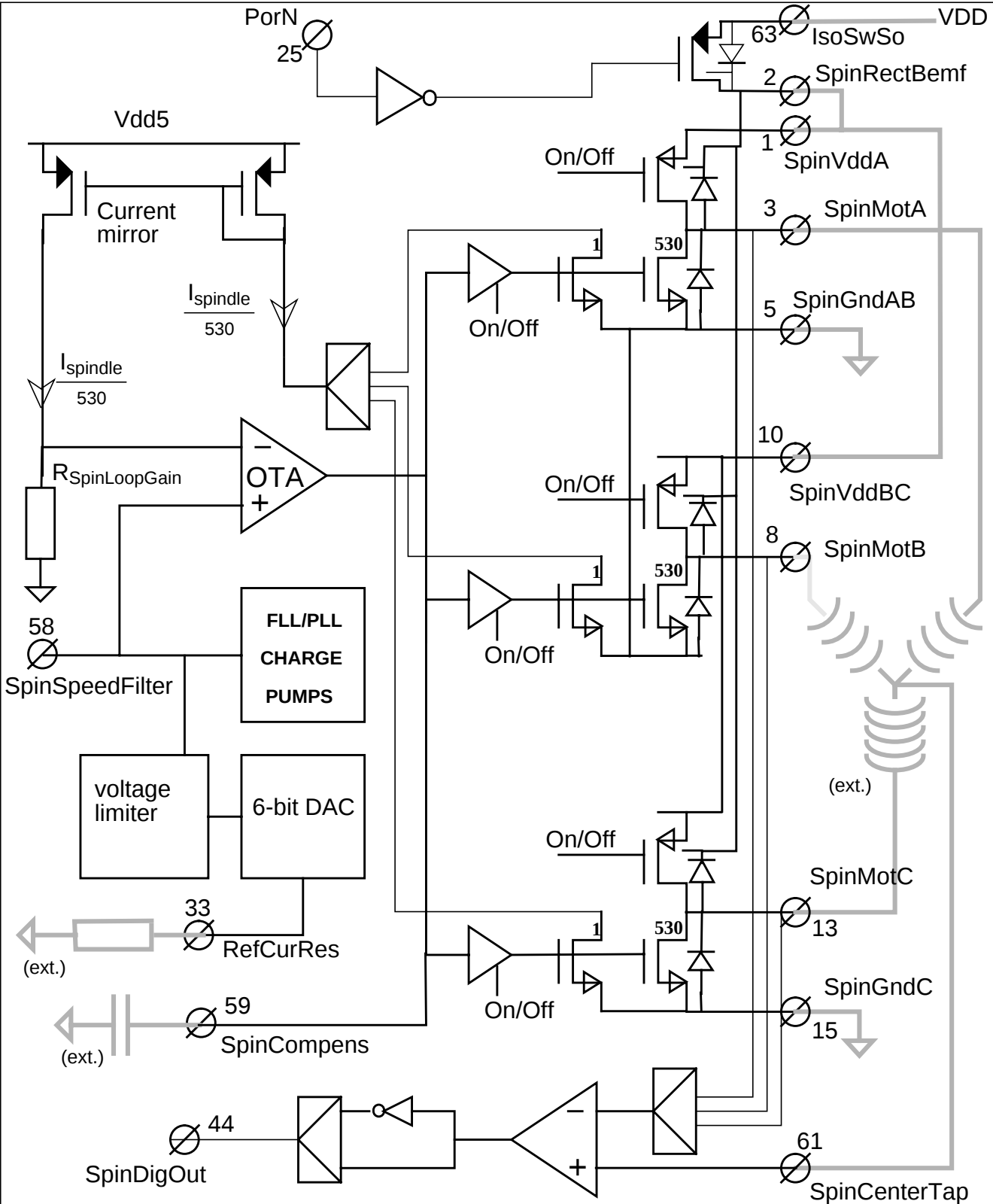
Fig.4 Spindle section diagram.
