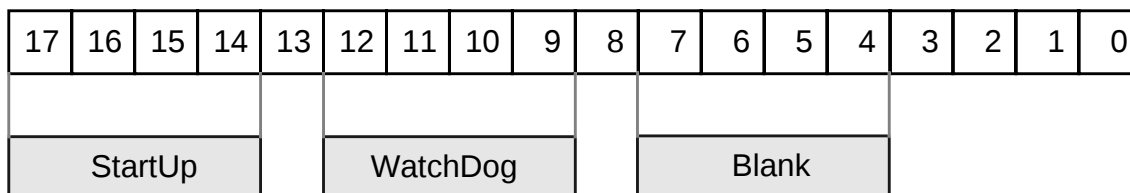
Fig.9 Timer 1 configuration.
