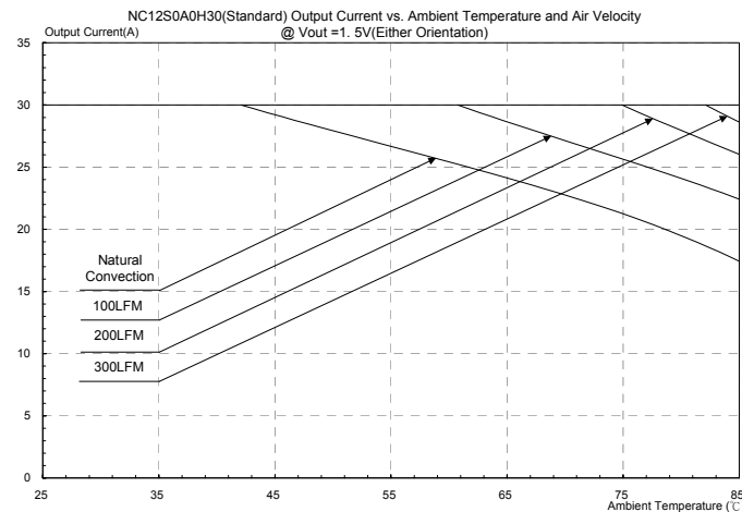
Figure 44: Output current vs. ambient temperature and air velocity @ Vout=1.5V(Either Orientation)
