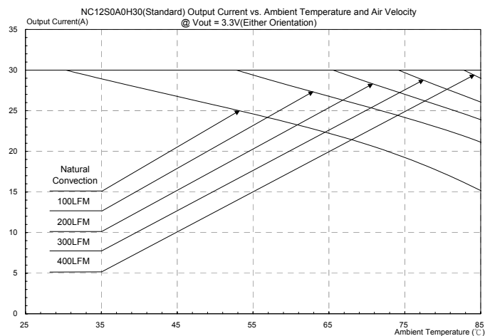
Figure 43: Output current vs. ambient temperature and air velocity @ Vout=3.3V(Either Orientation)
