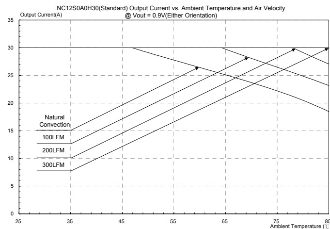
Figure 45: Output current vs. ambient temperature and air velocity @ Vout=0.9V(Either Orientation)
