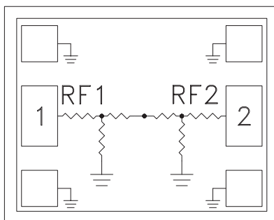
HMC651, HMC658
