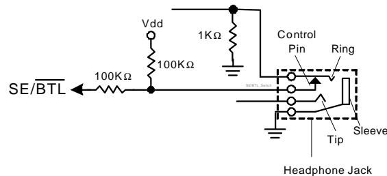
Figure 2: SE/BTL input selection by phonejack plug
