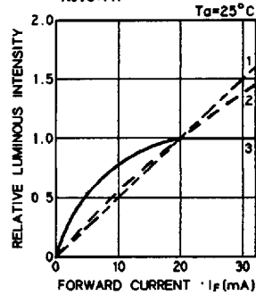
■ RELATIVE LUMINOUS INTENSITY vs. FORWARD CURRENT
