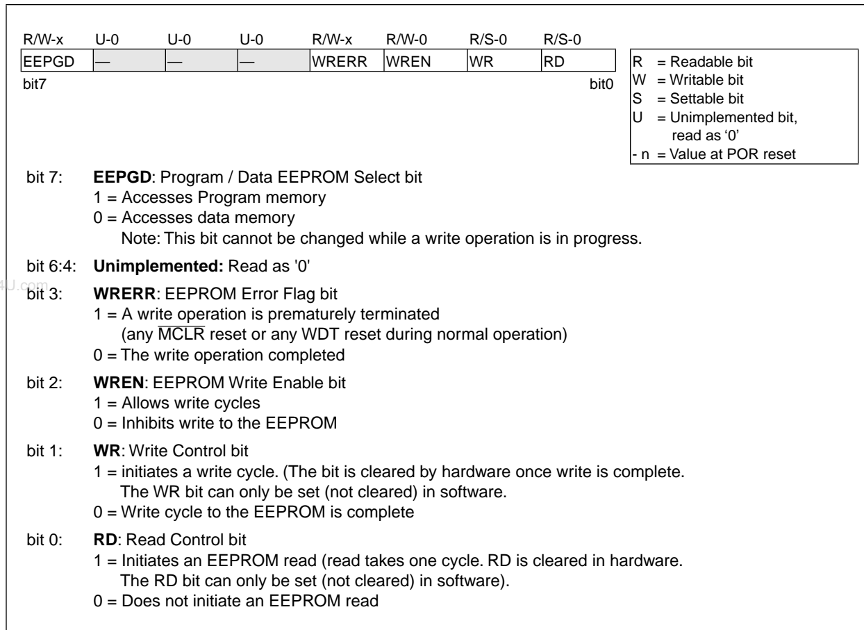
FIGURE 1: EECON1 REGISTER
