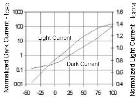
T_A - Ambient Temperature - ^\circ\text{C}
