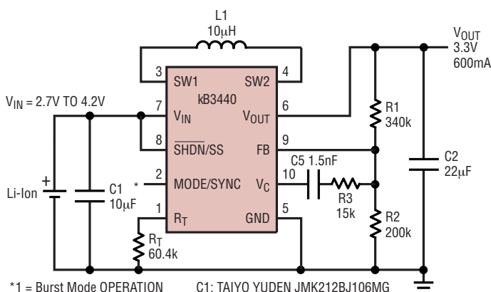
Li-Ion to 3.3V at 600mA Buck-Boost Converter
