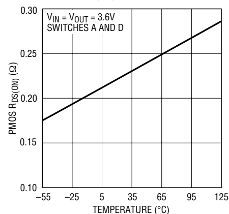
PMOS R_{DS(ON)}
