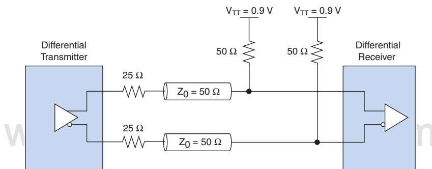
Figure 10–9. Differential SSTL-18 Class I Termination
