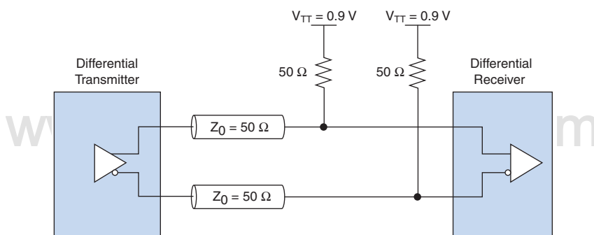
Figure 10-11. 1.8-V Differential HSTL Class I Termination
