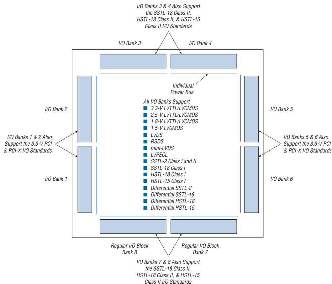
Figure 11–2. I/O Banks in EP2C20, EP2C35, EP2C50 &amp; EP2C70 Devices
