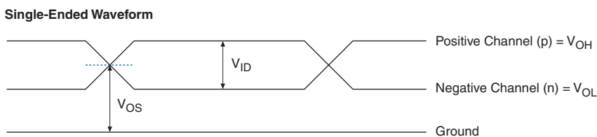
Figure 11-4. Receiver Input Waveforms for the LVDS Differential I/O Standard
