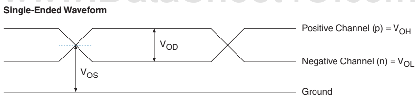
Figure 11-5. Transmitter Output Waveform for the LVDS Differential I/O Standard
