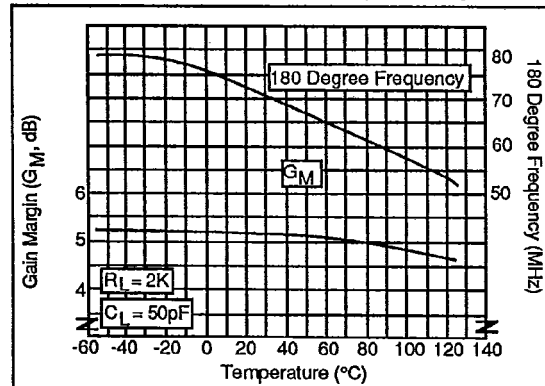
Gain Margin and 180 Degree Freq. vs Temp.
