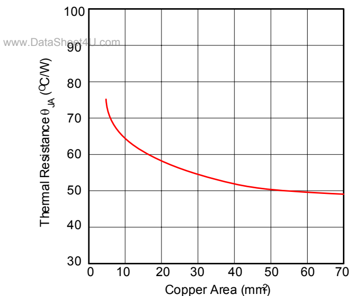
Figure 3. Thermal Resistance \theta_{JA} vs. Copper Area
