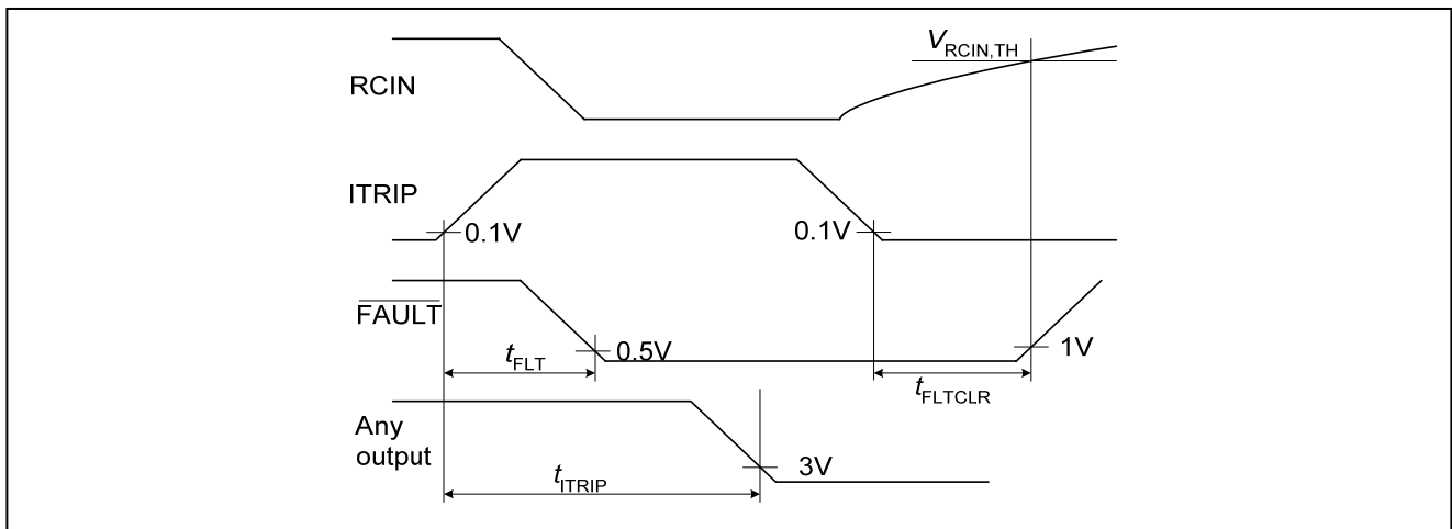
Figure 12: ITRIP-timing
