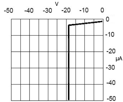
Reverse Current vs Reverse Voltage
