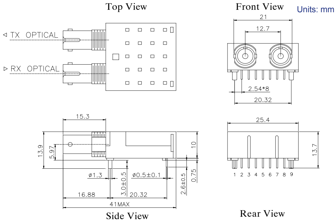
Package Diagram [C-1X-622-TDFB(3)-SST4]
