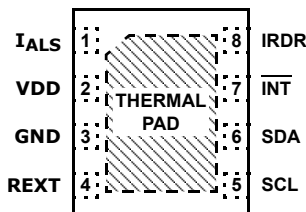
ISL29030A 8 LD ODFN (2.0X2.1X0.7MM) TOP VIEW
