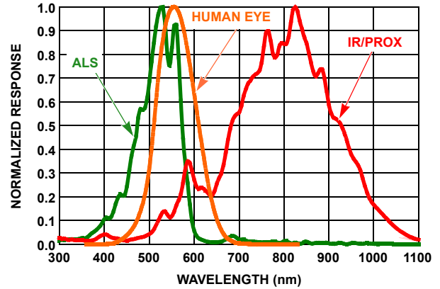
FIGURE 7. ISL29030A SENSITIVITY TO DIFFERENT WAVELENGTHS
