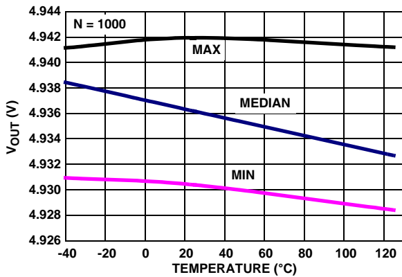
FIGURE 49. ISL28194 V_{OUT} HIGH vs TEMPERATURE, V_+ = 5V , R_L = 10k
