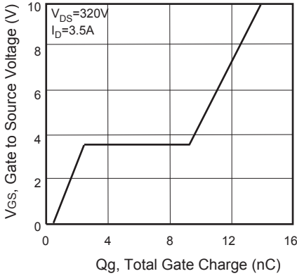
Figure 7. Gate Charge
