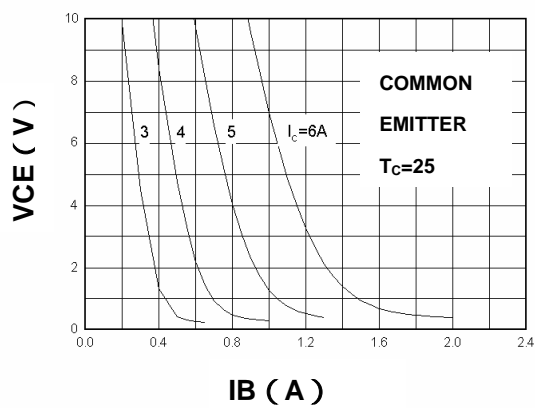
VCE - IB
