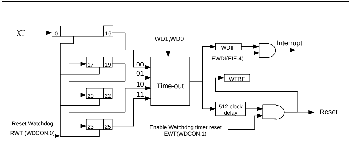
Figure 19. Watchdog Timer
