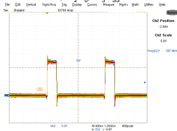
Fig. 11: Inductor node at 14A load Ch 2 :LX
