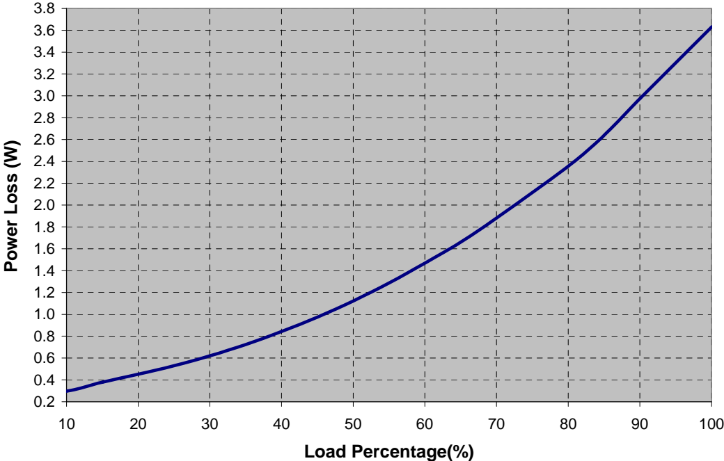
Fig.16: Power loss versus load current
