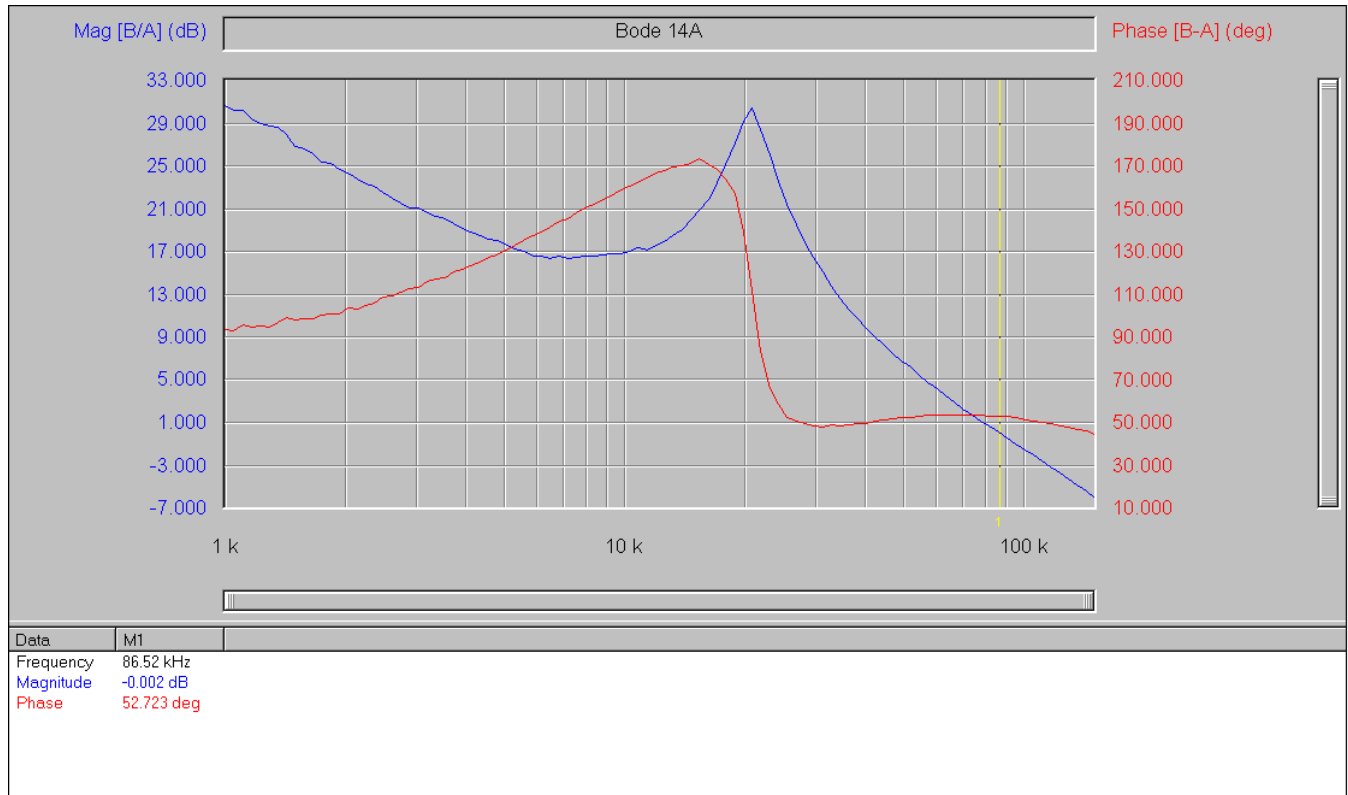
Fig. 14: Bode Plot at 14A load shows a bandwidth of 86kHz and phase margin of 53 degrees
