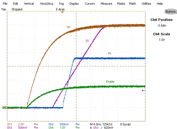
Fig. 7: Start up at 14A Load Ch 1 :V in , Ch 2 :V o , Ch 3 :V SS , Ch 4 :Enable
