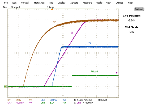
Fig. 8: Start up at 14A Load, Ch 1 :V in , Ch 2 :V o , Ch 3 :V SS , Ch 4 :V PGGood
