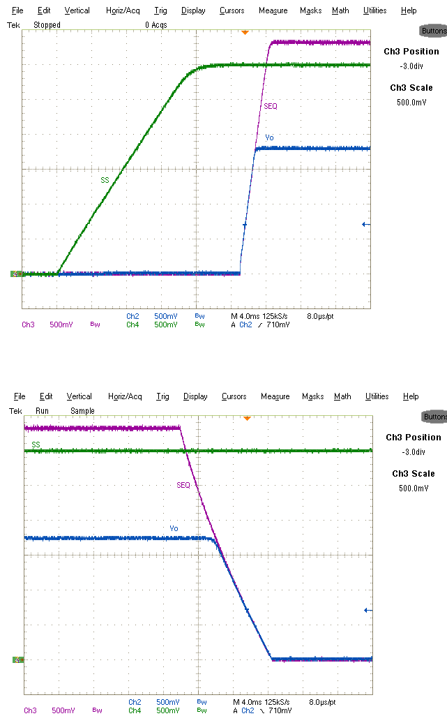
Fig. 18: Simultaneous Tracking a 3.3V input at power-up and shut-down Ch2: SEQ Ch3:Vo Ch4: SS (1.8V)
