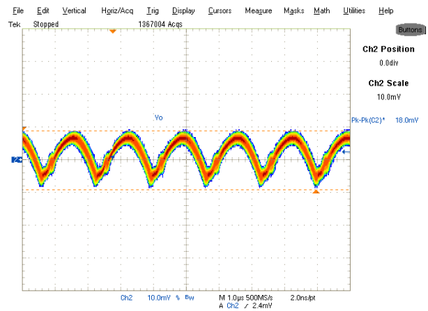
Fig. 10: Output Voltage Ripple, 14A load Ch 2 : V out
