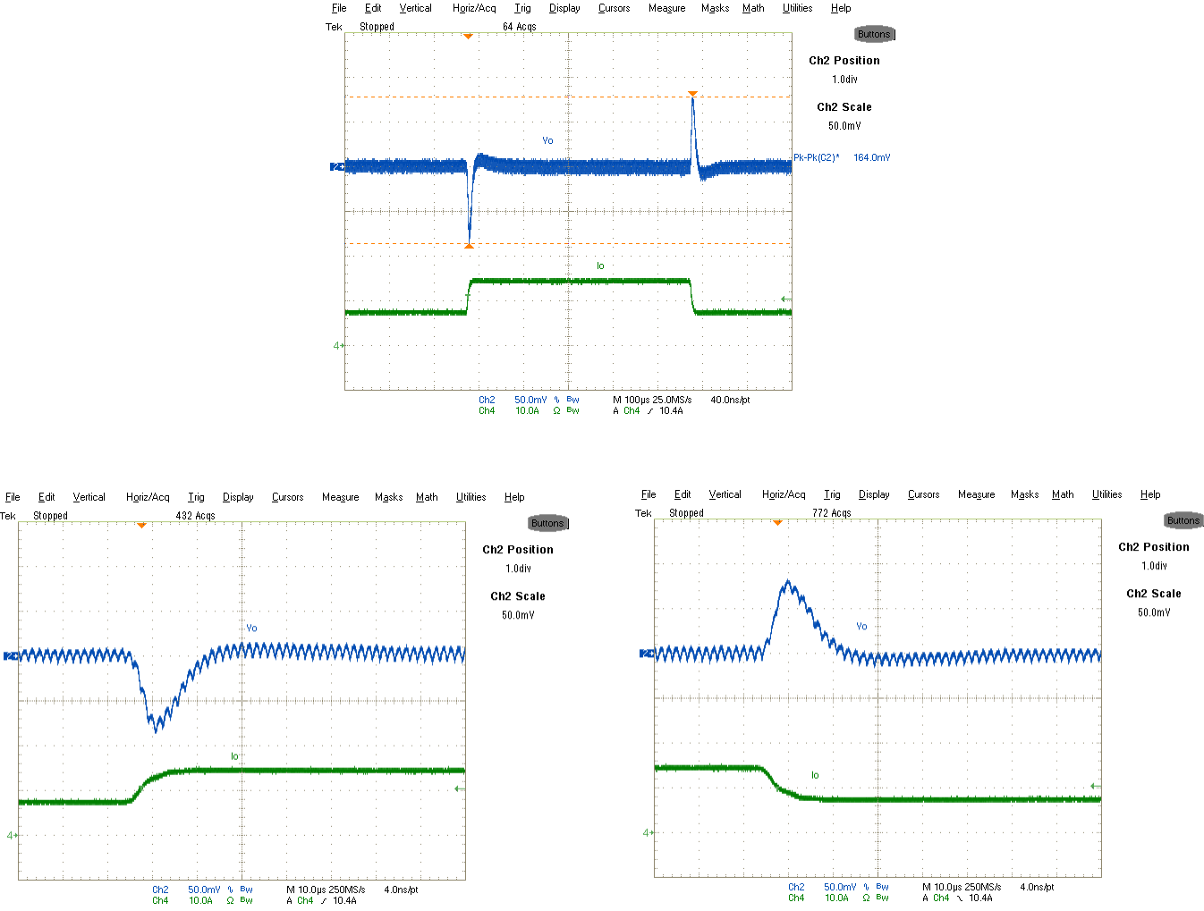
Fig. 13: Transient Response, 7A to 14A step 2.5A/μs Ch 2 :V out , Ch 4 :I out
