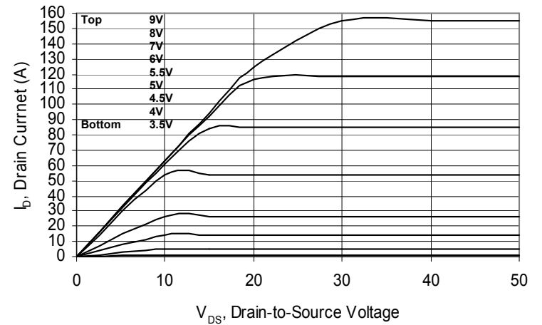
Extended Typical Output Characteristics
