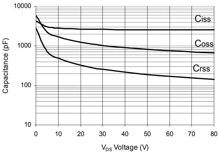
V_{DS} vs. Capacitance
