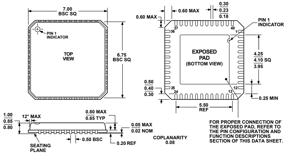
COMPLIANT TO JEDEC STANDARDS MO-220-VKGD-2 Figure 34. 48-Lead Lead Frame Chip Scale Package [LFCSP_VQ] 7 mm × 7 mm Body, Very Thin Quad (CP-48-12) Dimensions shown in millimeters
