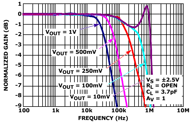
FIGURE 16. GAIN vs FREQUENCY vs V_{OUT} , R_L = \text{OPEN}
