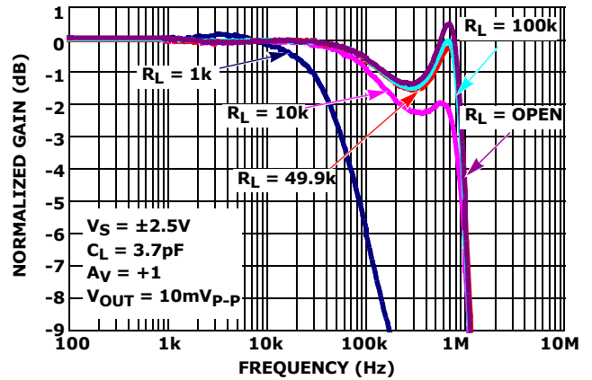
FIGURE 14. GAIN vs FREQUENCY vs R_L , V_S = \pm 2.5V
