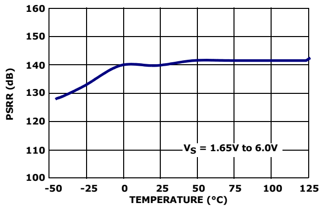
FIGURE 24. PSRR vs TEMPERATURE
