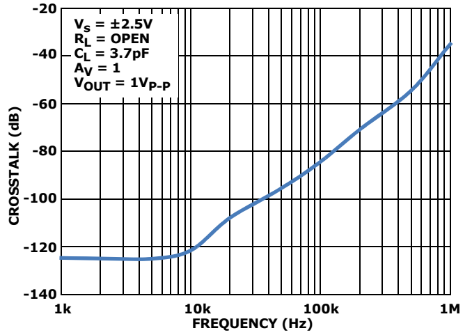
FIGURE 31. CROSSTALK vs FREQUENCY, V_S = \pm 2.5V
