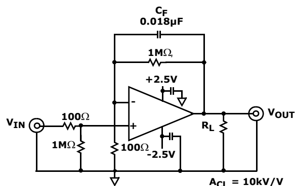
FIGURE 41. HIGH GAIN, PRECISION DC-COUPLED AMPLIFIER
