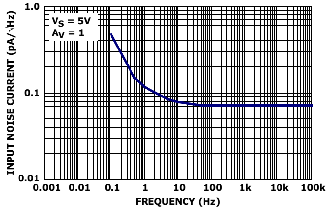
FIGURE 10. INPUT NOISE CURRENT DENSITY vs FREQUENCY
