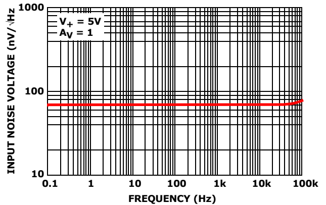
FIGURE 45. SIMULATED INPUT NOISE VOLTAGE DENSITY vs FREQUENCY
