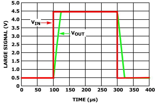
FIGURE 51. SIMULATED LARGE SIGNAL STEP RESPONSE (4V)
