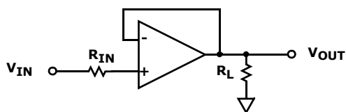
FIGURE 40. INPUT CURRENT LIMITING
