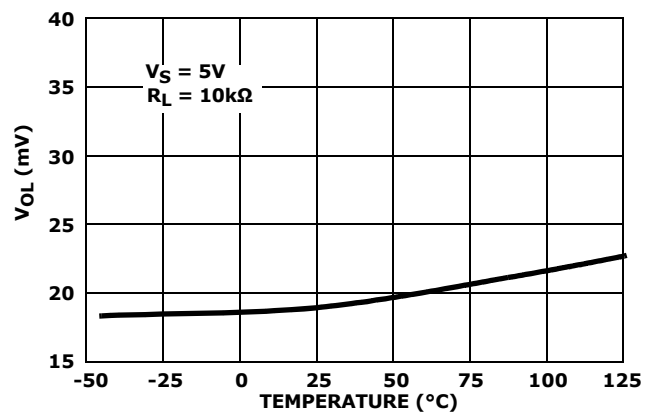
FIGURE 29. V_{OL} vs TEMPERATURE
