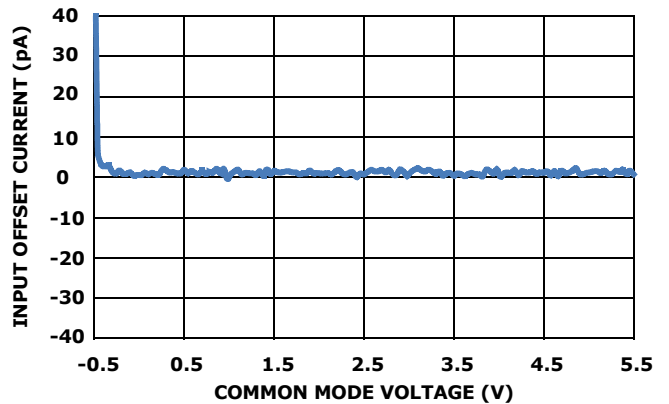
FIGURE 35. I_{OS} vs V_{CM}
