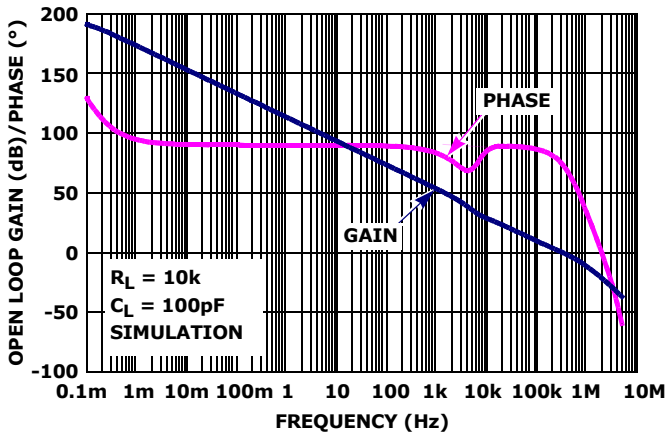
FIGURE 11. FREQUENCY RESPONSE vs OPEN LOOP GAIN, R_L = 10k\Omega
