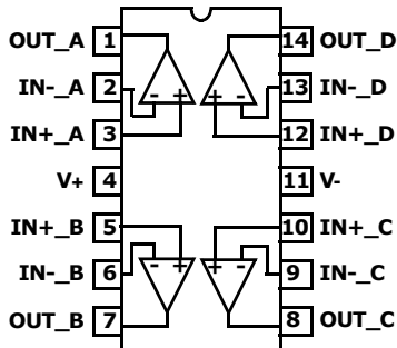
ISL28433 (14 LD SOIC) TOP VIEW
