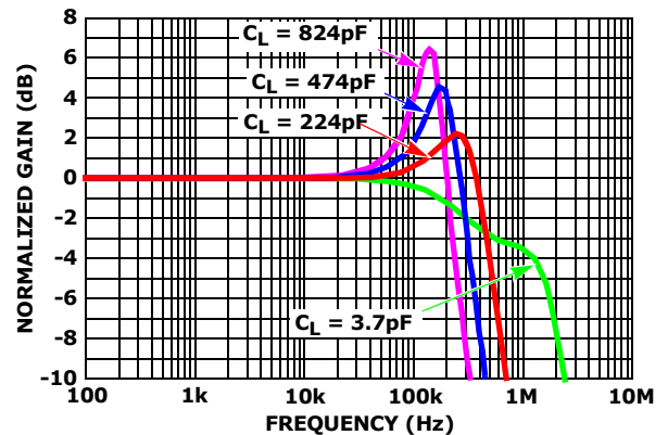
FIGURE 49. SIMULATED GAIN vs FREQUENCY vs C_L
