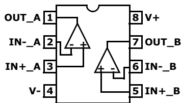
ISL28233 (8 LD MSOP, SOIC) TOP VIEW
