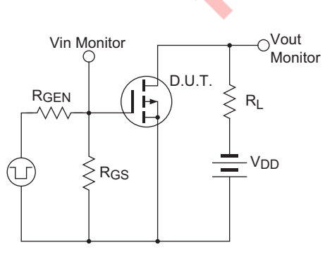
Switching Time Measurement Circuit
