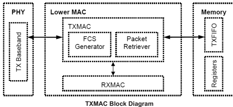
TXMAC Block Diagram
