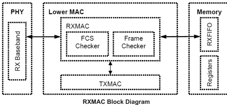
RXMAC Block Diagram
