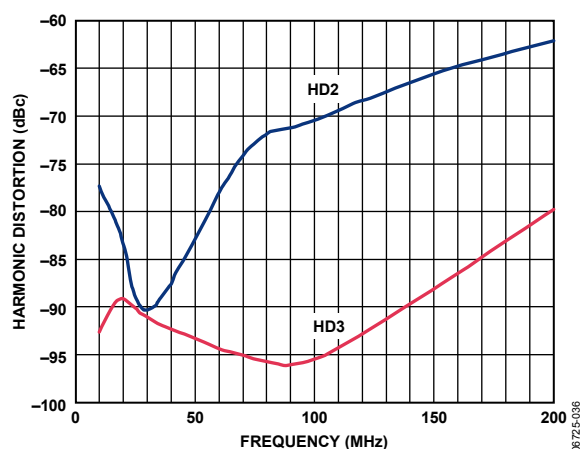
Figure 35. Harmonic Distortion vs. Frequency of Single-Ended-to-Differential Conversion
