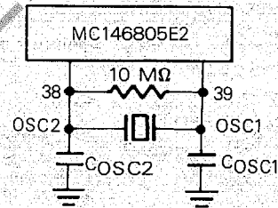
Crystal Oscillator Connections
