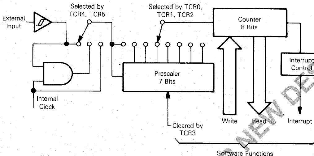
FIGURE 19 — TIMER BLOCK DIAGRAM
