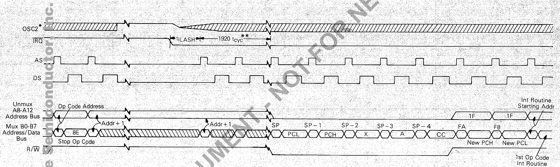
FIGURE 8 - INTERRUPT RECOVERY FROM STOP INSTRUCTION: TIMING
