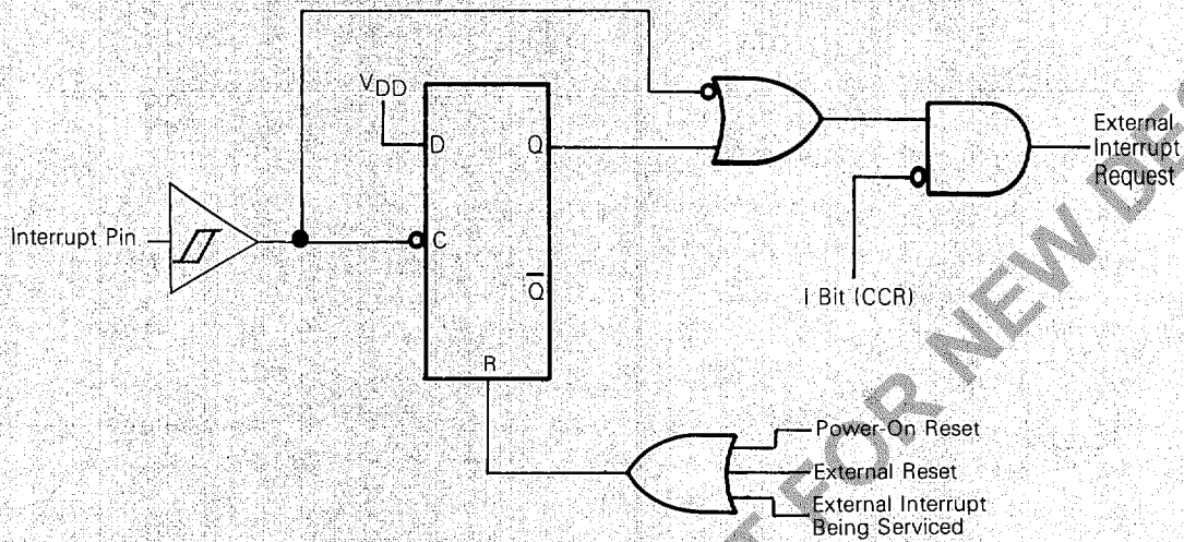
(a) Interrupt Functional Diagram
