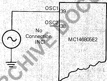
FIGURE 10 — EXTERNAL CLOCK CONNECTION
