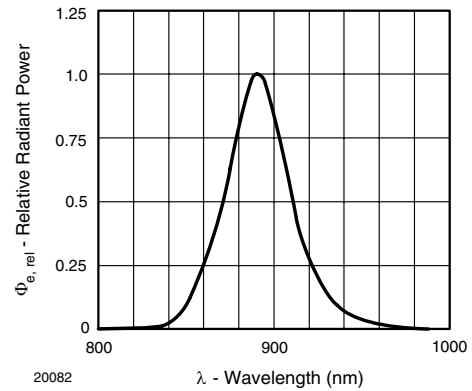
Figure 7. Relative Radiant Power vs. Wavelength
