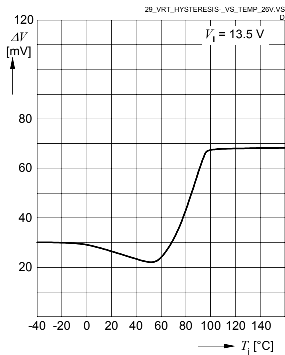
Reset Hysteresis versus Junction Temperature T_j (2.6V-Version)
