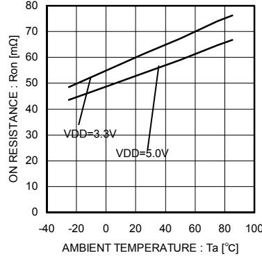
Fig.27 ON resistance
