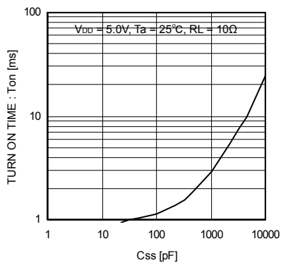
Fig.44 Turn On time (vs. Ccss)
