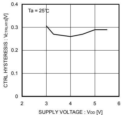
Fig.34 CTRL hysteresis voltage
