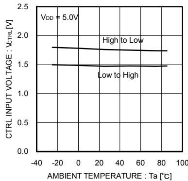
Fig.33 CTRL input voltage
