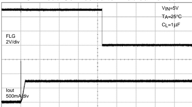
3 Ω Load Connected to Enabled Device
