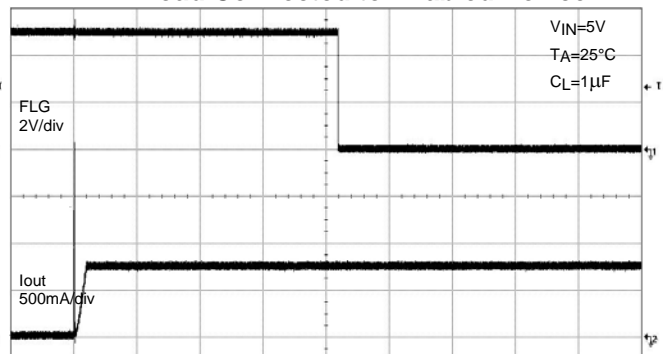
2 Ω Load Connected to Enabled Device
