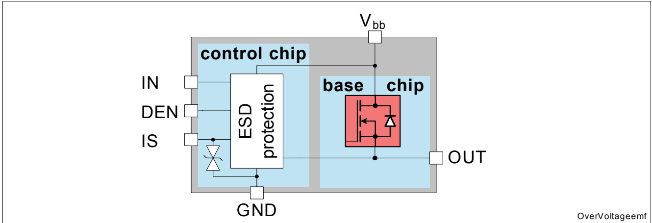
Figure 18 Over-Voltage Protection
