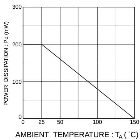
Fig.2 Derating curve
