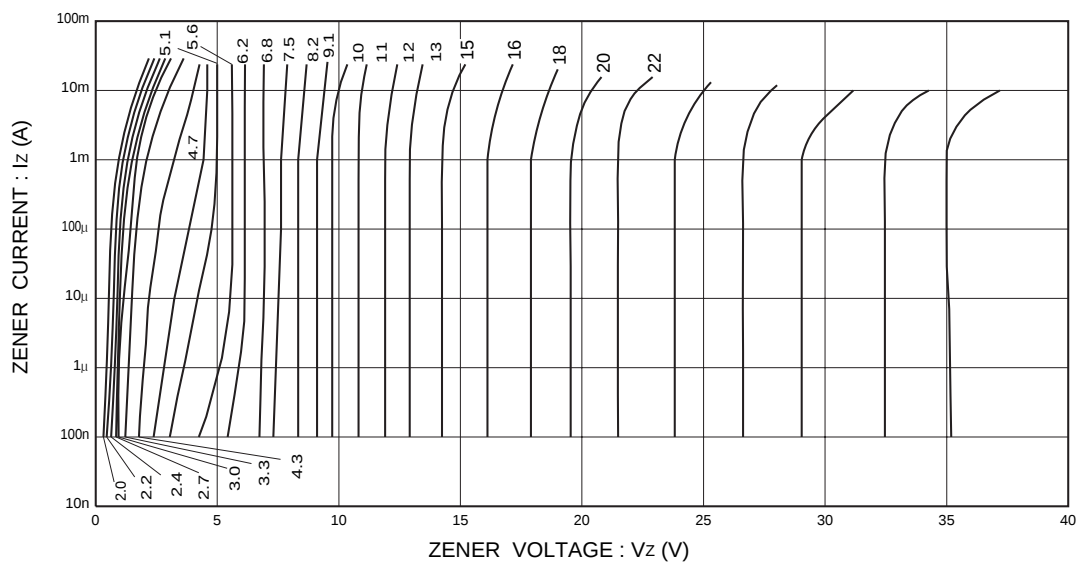
Fig.1 Zener voltage characteristics
