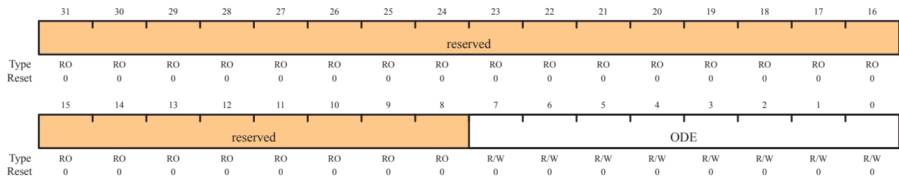
GPIO Open Drain Select (GPIODR)
