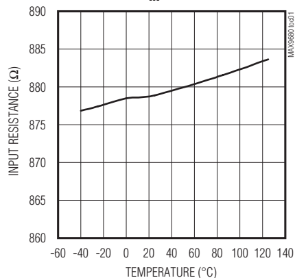
INPUT RESISTANCE vs. TEMPERATURE V_{IN} = 0.4V
