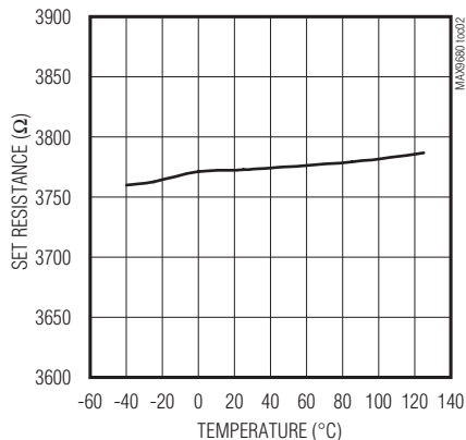
SET RESISTANCE vs. TEMPERATURE
