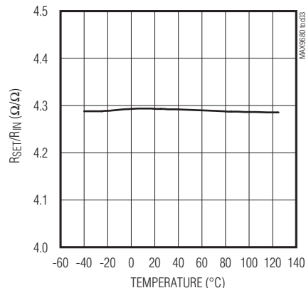
R SET /R IN vs. TEMPERATURE
