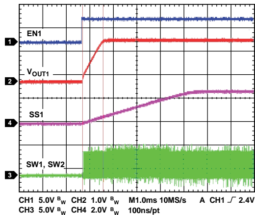
Figure 44. Soft Start, Channel 1: V_{OUT} = 1.8\text{ V} , C_{SS1} = 10\text{ nF}
