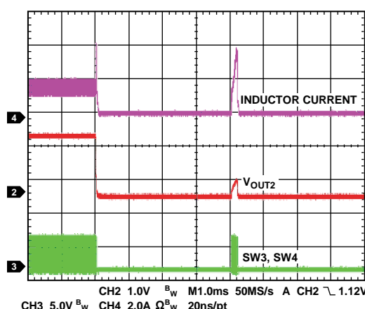
Figure 46. Current Limit Entry, Channel 2: V_{OUT} = 1.8\text{ V} , 2 A Configuration, f_{sw} = 600\text{ kHz}
