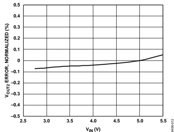
Figure 12. Line Regulation, Channel 2: Load Current = 3 A and f_{SW} = 600\text{ kHz}
