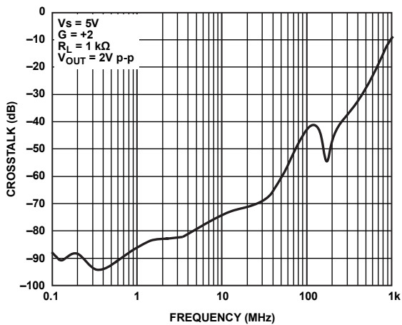
Figure 45. All-Hostile Crosstalk (Output-to-Output) vs. Frequency
