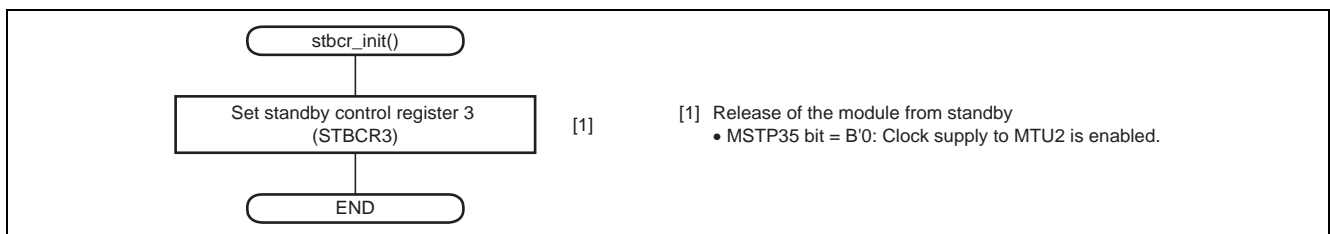
Figure 12 Initialization: Release from Standby
