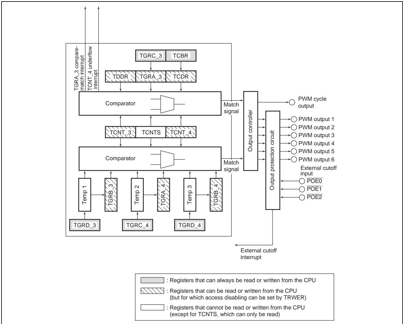
Figure 3 Block Diagram of Channels 3 and 4 in Complementary PWM Mode
