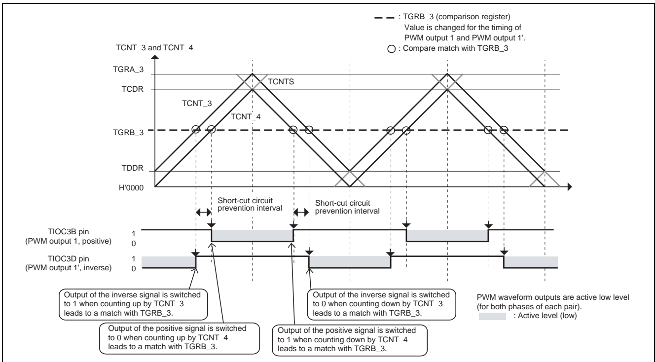
Figure 6 Output of PWM Waveforms in Complementary PWM Mode
