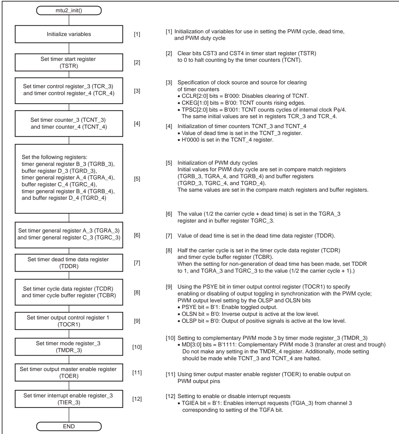
Figure 13 Initialization of MTU2
