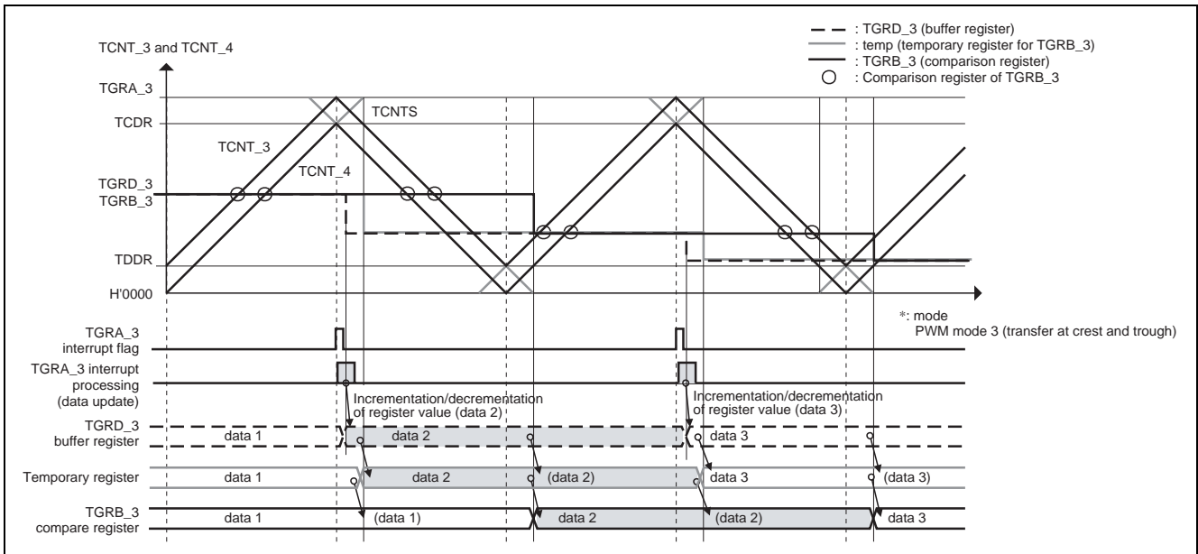
Figure 7 Timing of Updating the PWM Duty Cycle
