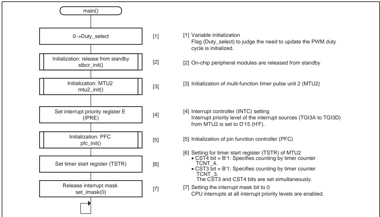
Figure 11 Processing by Function main
