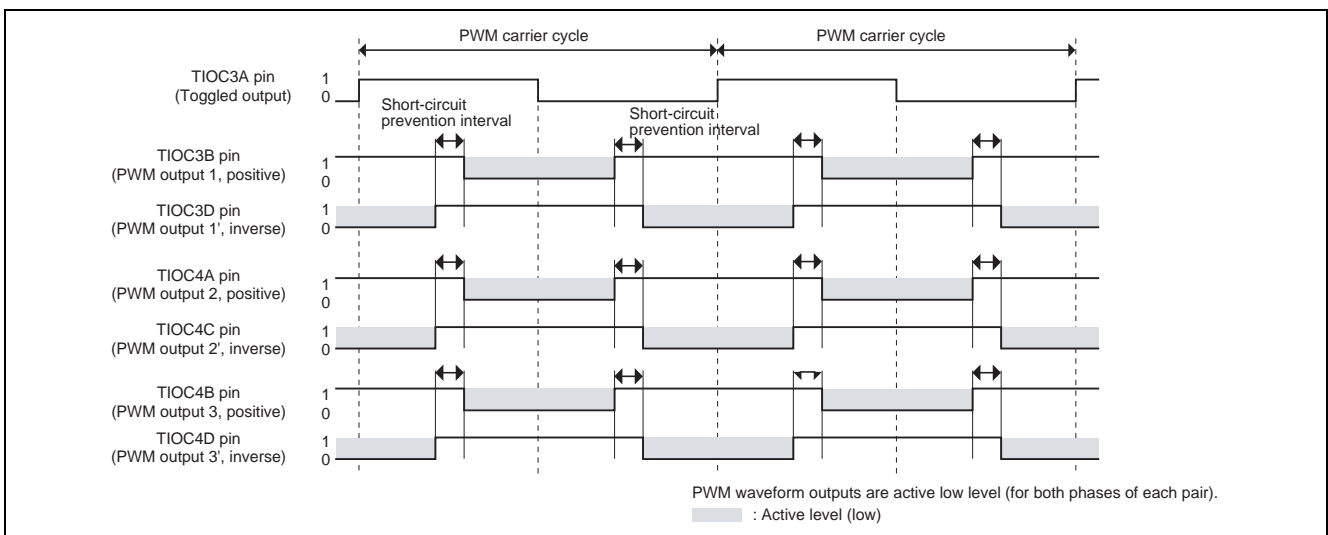
Figure 4 Output Waveforms in Complementary PWM Mode Operation
