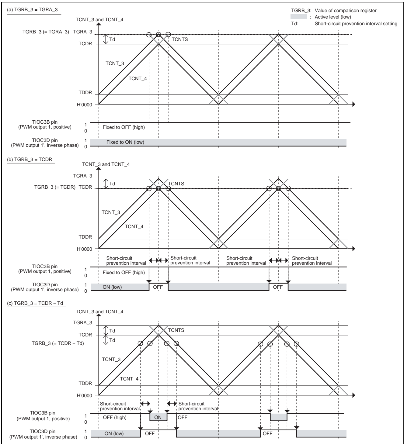
Figure 9 Examples of PWM Waveform Output (1)
