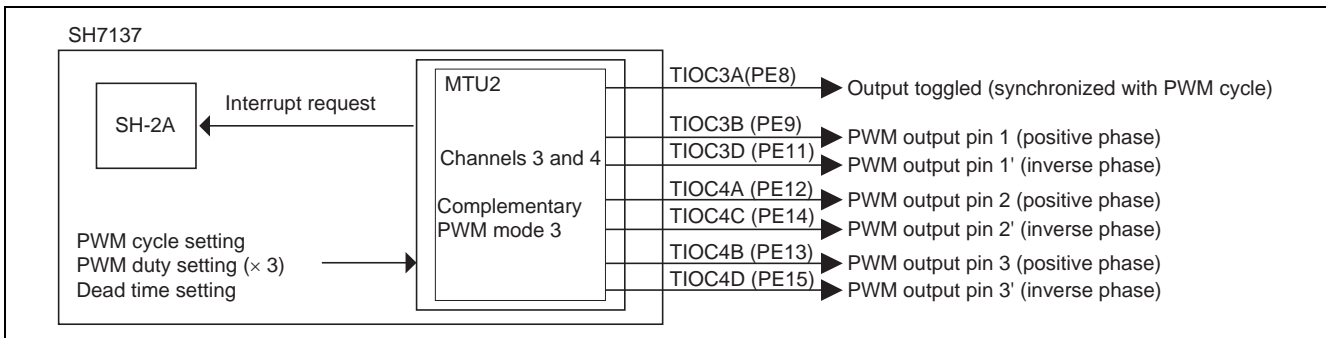
Figure 1 Three-Phase Output of Complementary PWM (Complementary PWM Mode 3)
