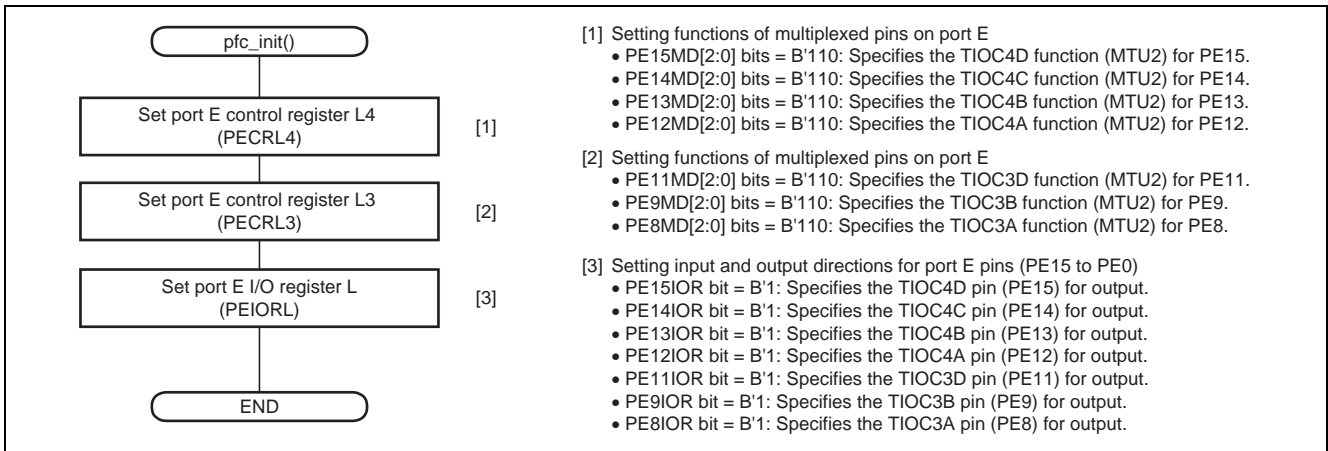
Figure 14 Initialization of Pin Function Controller (PFC)
