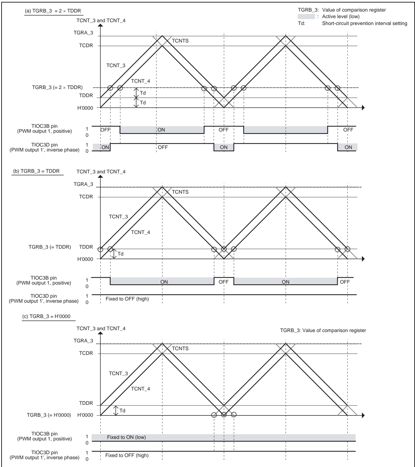
Figure 10 Examples of PWM Waveform Output (2)
