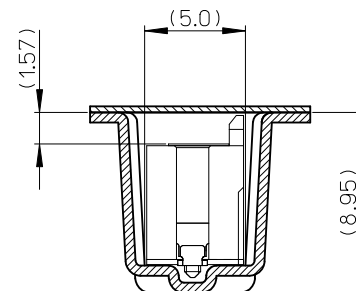
SECT. X-X
