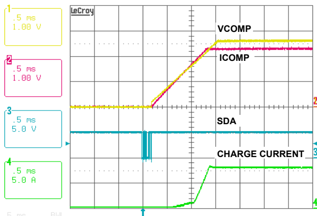
FIGURE 15. CHARGE ENABLE: WRITE 1F80 (8.064A) TO CHARGE CURRENT REGISTER
