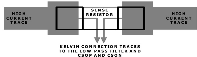
FIGURE 33. CURRENT SENSE RESISTOR LAYOUT
