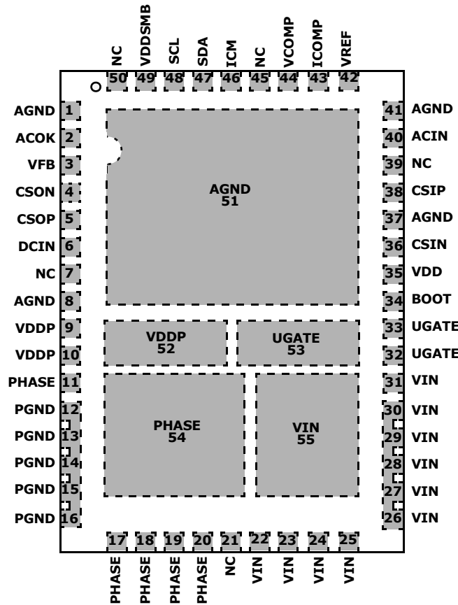
ISL95871C (50 LD 5x7 QFN) TOP VIEW
