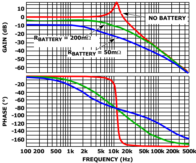
FIGURE 31. FREQUENCY RESPONSE OF THE LC OUTPUT FILTER
