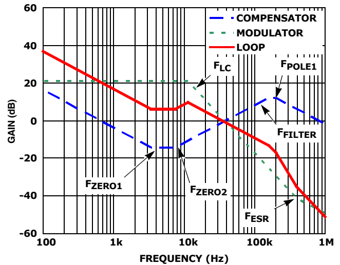
FIGURE 32. ASYMPTOTIC BODE PLOT OF THE VOLTAGE CONTROL LOOP GAIN
