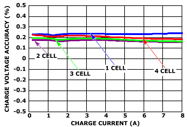
FIGURE 10. CHARGE VOLTAGE ACCURACY
