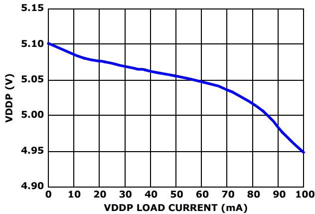
FIGURE 5. VDDP LOAD REGULATION
