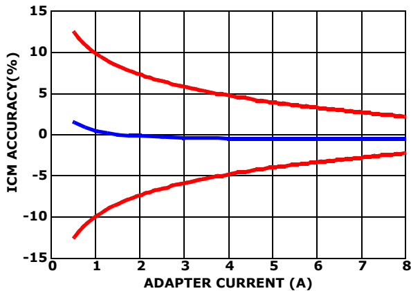
FIGURE 7. ICM ACCURACY vs AC-ADAPTER CURRENT
