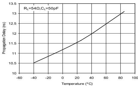
Driver Average Propagation Delay vs Temperature (SP3086-SP3088)
