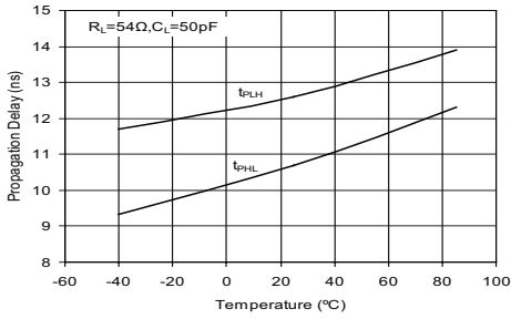
Driver Propagation Delay vs Temperature (SP3086-SP3088)
