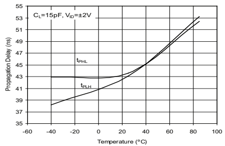
Receiver Propagation Delay vs Temperature (SP3086-SP3088)
