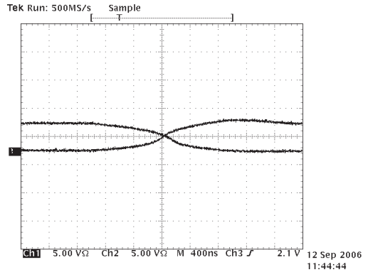
Driver output Waveform Low to High (SP3080-SP3082)
