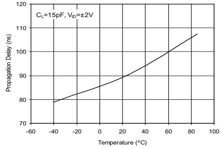
Receiver Average Propagation Delay vs Temperature (SP3080-SP3082)
