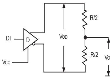
Driver DC Test Circuit
