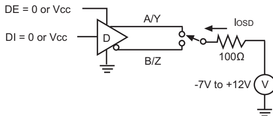
Driver Short Circuit Current Limit Test Circuit
