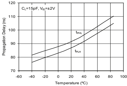
Receiver Propagation Delay vs Temperature (SP3080-SP3082)
