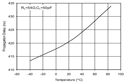
Driver Average Propagation Delay vs Temperature (SP3083-SP3085)
