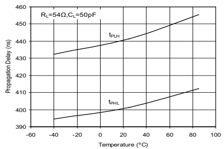
Driver Propagation Delay vs Temperature (SP3083-SP3085)
