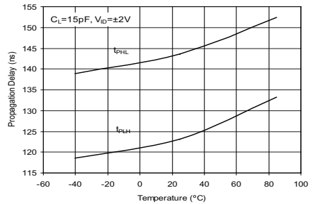
Receiver Propagation Delay vs Temperature (SP3083-SP3085)
