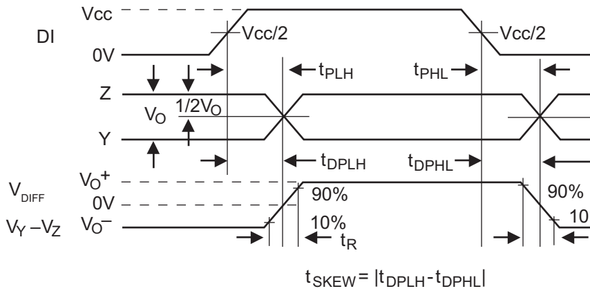
Driver Propagation Delay Time Test Circuit and Timing Diagram
