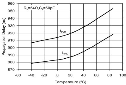
Driver Propagation Delay vs Temperature (SP3080-SP3082)
