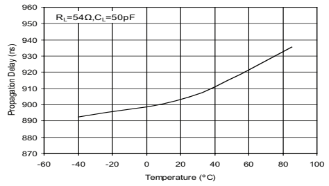
Driver Average Propagation Delay vs Temperature (SP3080-SP3082)
