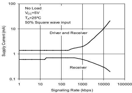
Supply Current vs Signaling Rate (SP3086-SP3088)
