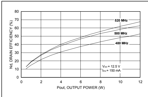
Figure 19. Drain efficiency vs. output power
