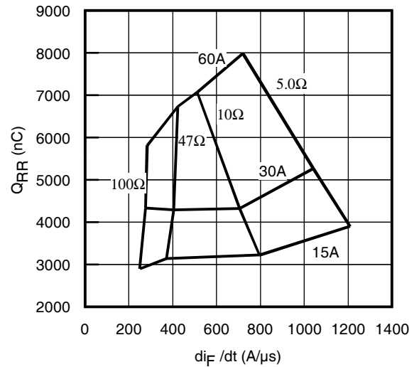
Fig. 20 - Typ. Diode Q_{RR} vs. di/dt V_{CC} = 600\text{V} ; V_{GE} = 15\text{V} ; T_J = 150^\circ\text{C}
