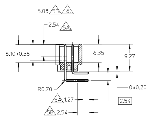
SECTION E-E
