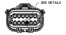
REAR VIEW MALE CONNECTOR ASSEMBLY
