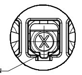
DETAIL 1 SCALE 10:1 INSTALL SEAL PLUG INTO RECEPTACLE ASSEMBLY AS SHOWN ONLY SEE NOTE 7
