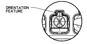
DETAIL 2 SCALE 10:1 INSTALL SEAL PLUG INTO BLADE ASSEMBLY AS SHOWN ONLY SEE NOTE 7
