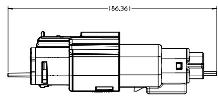
VIEW SHOWING SEAL PLUG ASSEMBLED WITH MOLEX CONNECTORS SEE NOTE 5 SCALE 2:1
