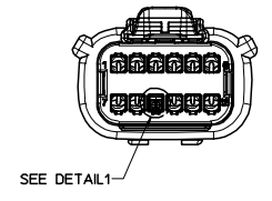
REAR VIEW FEMALE CONNECTOR ASSEMBLY
