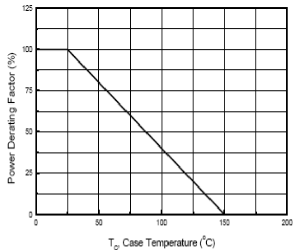
Fig. 4 Power Derating
