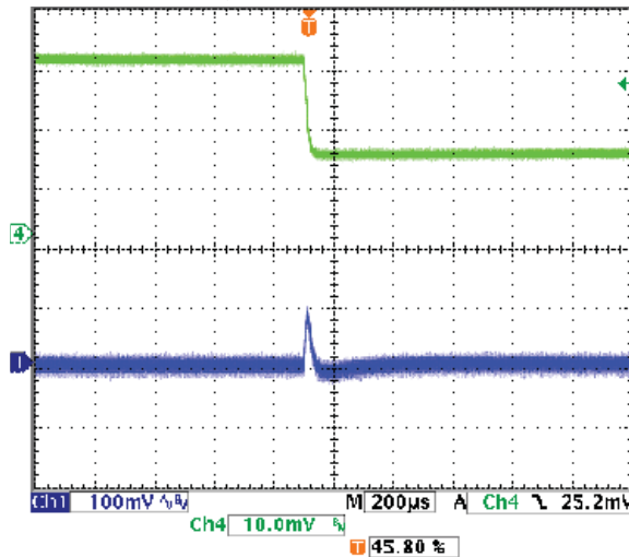
Step Load Transient Response (V IN =5V, V OUT =1.5V, Load=0, I OUT =16A to 8A) Trace 1=V OUT , 100 mV/div. Trace 4=I OUT , 5A/div.
